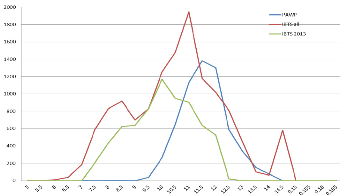
Figure 4-14: Sprat Length frequency distribution in average numbers caught per hour. Blue PAWP: number of tows =8; Red all the IBTS tows in the vicinity: number of tows=43; Green only the 2013 IBTS: number of tows=2.
